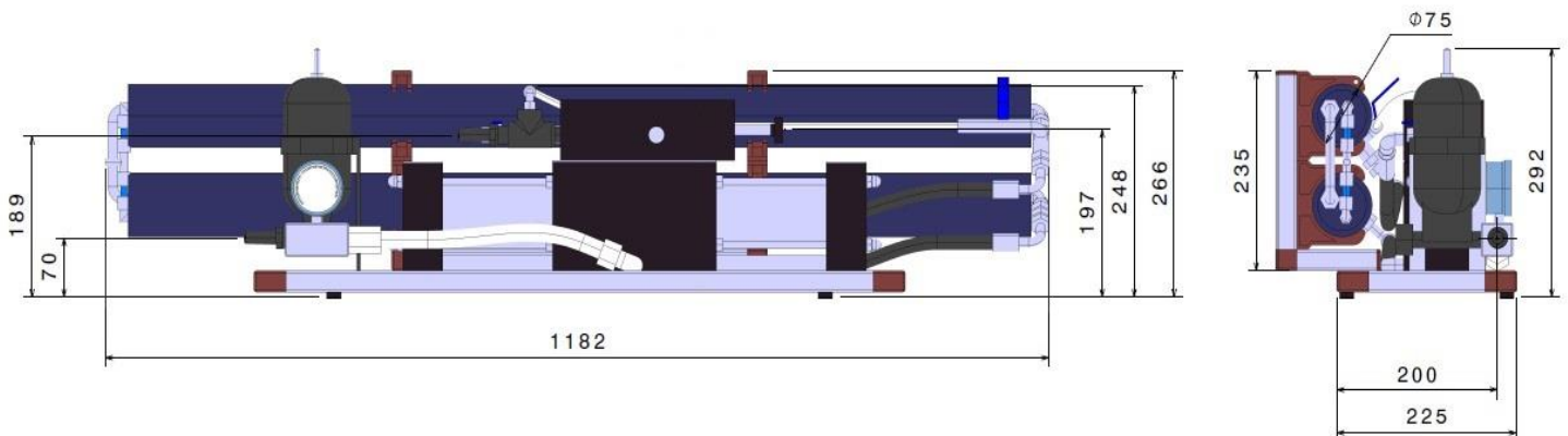
WATERMAKER DIMENSIONS FIG. 3-4
