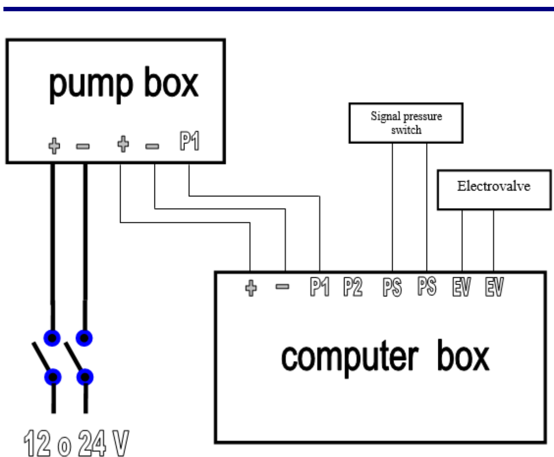
WIRING LOGIC SCHEME 12-24 VDC
