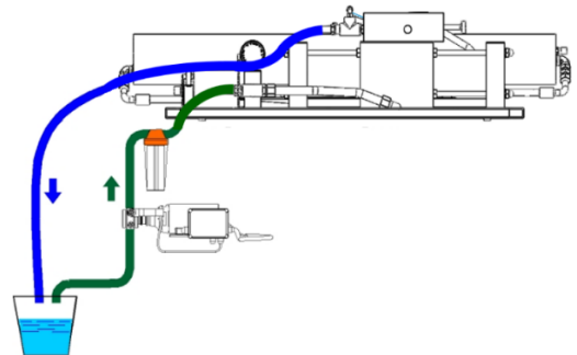
HYDRAULIC SCHEME FOR WINTERIZING PROCEDURE FIG. 6-2
