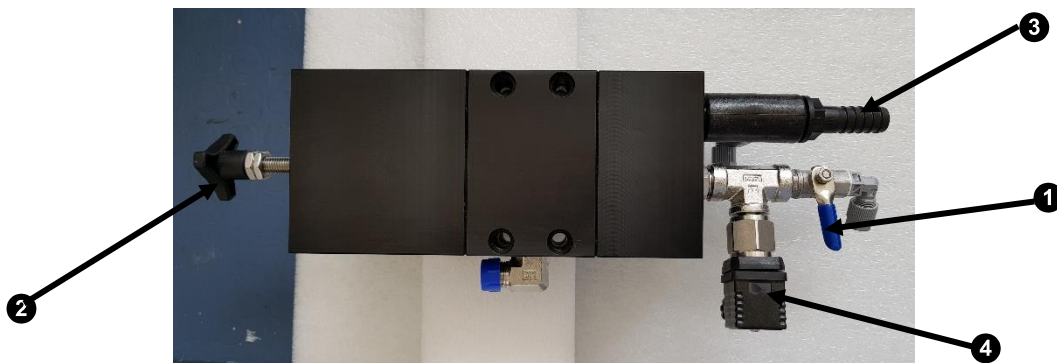
WATERMAKER GROUP (TOP VALVE VIEW) FIG. 3-8
